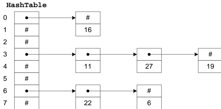
Figure 3-1: A Hash Table
