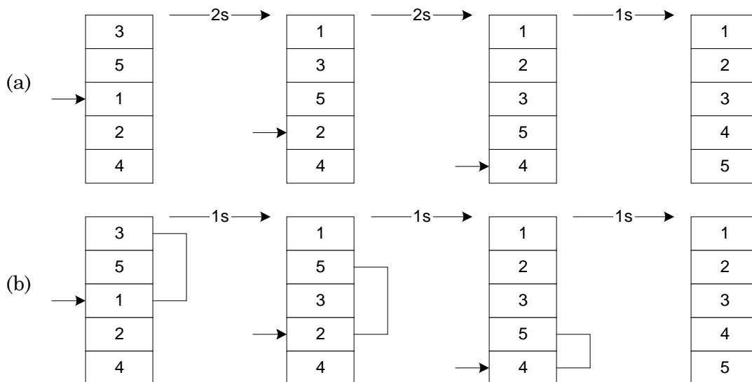
Figure 2-2: Shell Sort
