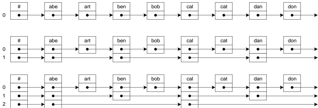
Figure 3-8: Skip List Construction
