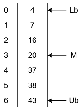
Figure 1-1: An Array
